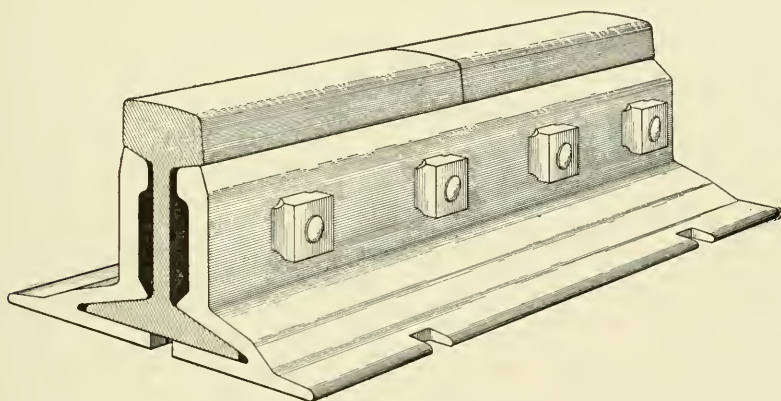
Fig. 226. Continuous Rail Joint
